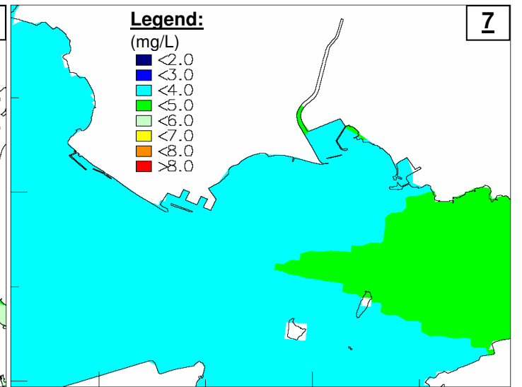
Scenario 2b (Assumed BOD 5 Level in the PPSTW Effluent: 180mg/L)
